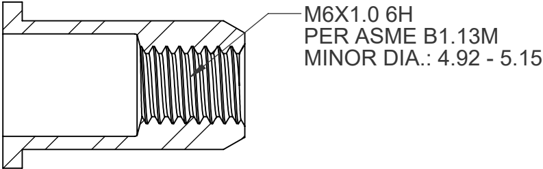
SECTION A-A SCALE 2.5 : 1
