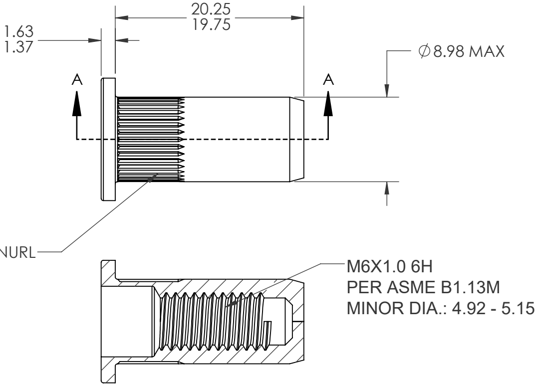
SECTION A-A SCALE 2.5 : 1
