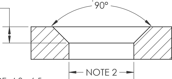
HOLE DETAIL
