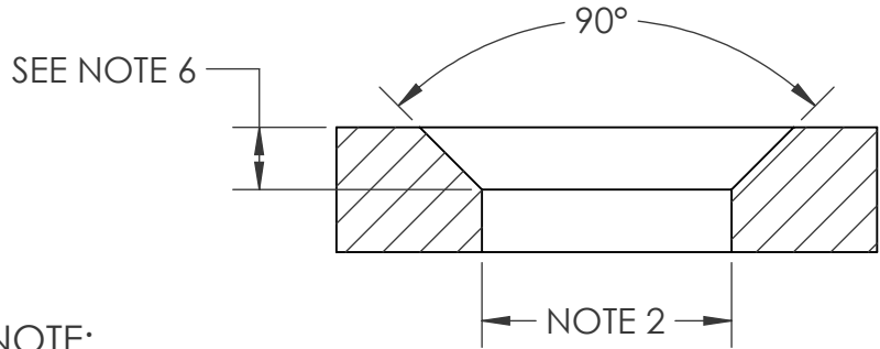
HOLE DETAIL
