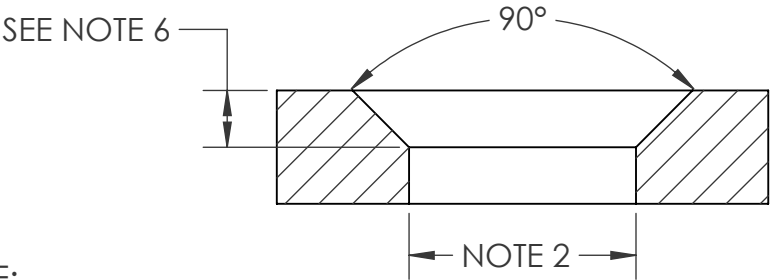
HOLE DETAIL
