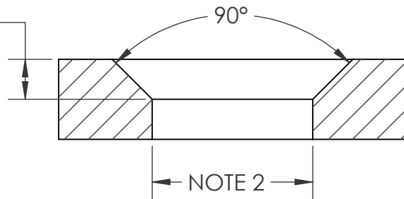
HOLE DETAIL
