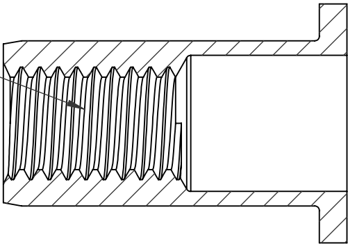
SECTION A-A SCALE 3.5 : 1
